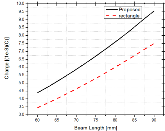
Figure 12. The generated charge versus beam length at W=36\text{mm} , t_p=0.4\text{mm}
